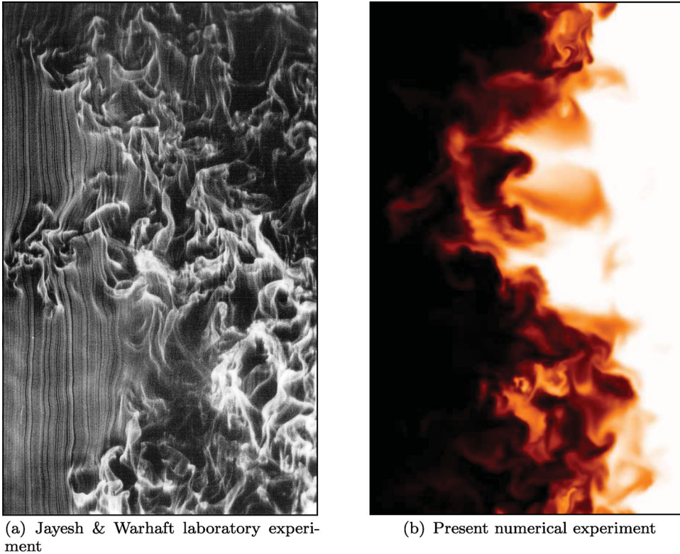
Figure 3. Comparison between a laboratory visualization by Jayesh and Warhaft ([19] Figure 8(a)) and present simulation: (a) Smoke-wire (streaklines) visualization of the shearless mixing layer without thermal stratification, wind tunnel experiment, and side view at a distance from the grid equivalent to our time evolution at t/\tau \approx 9 . The flow is from top to bottom and Re_\lambda = 130 [19]. The energy ratio can be estimated as of order 10^2 because the turbulence level in the part of the flow out of the grid (on the right in this picture) has a ratio velocity rms/mean velocity less than 0.25%. It should be noted that this visualization is not exactly the equivalent of the one in panel (b). In fact, the equivalent view would have been a tunnel cross section at a constant x . (b) Pseudo-colour of the passive scalar concentration along the mixing layer in a central portion of the domain at t/\tau = 10 , initial Re_\lambda = 150 , the initial energy ratio is equal to 6.7.
