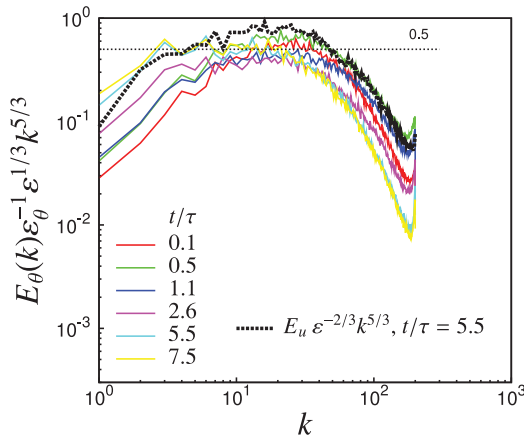
(b) 3D mixing, Re_\lambda = 150
