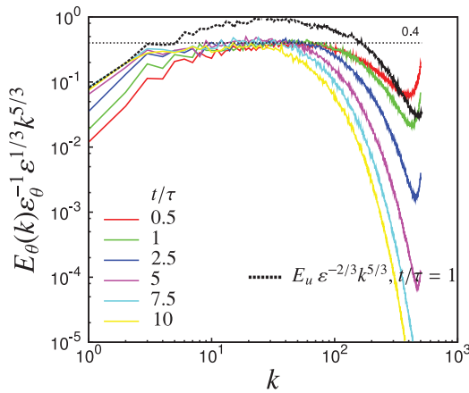
(c) 3D mixing, Re_\lambda = 250
